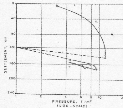
Fig. 10. Hydro-test on Tank
