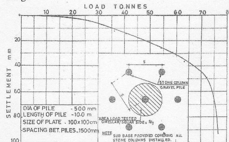
Fig. 5. Load Test on Single Granular Pile
