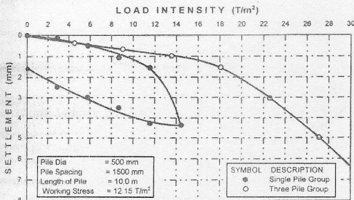
Fig. 7. Comparison of Load Test Results on Single Granular Pile and Group of Three Granular Piles
