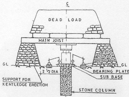
Fig. 2. Test Arrangement for Load Test on Single Granular Pile
