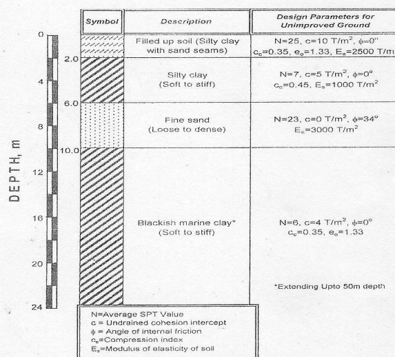
Fig. 1. Design Profile for Unimproved Ground
