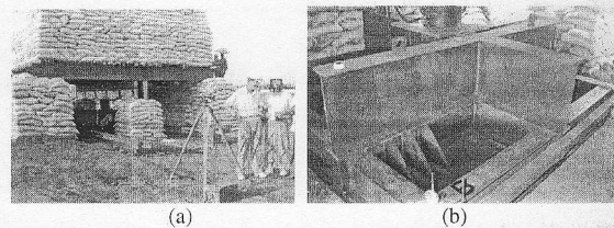
Fig. 4. Load Test Arrangement on Group of Granular Piles (a) Dead Load Kentledge (b) Close-up View of Test Plate and Dial Gauge
