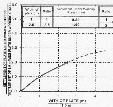
Fig. 8. Plate Size Versus Settlement
